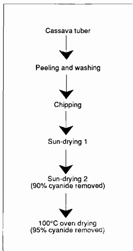
Figure 9.15. Flow chart for preparation of detoxified cassava flour from high-cyanide cassava varieties
