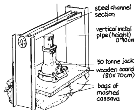
Figure 9.19. Hydraulic jack press
