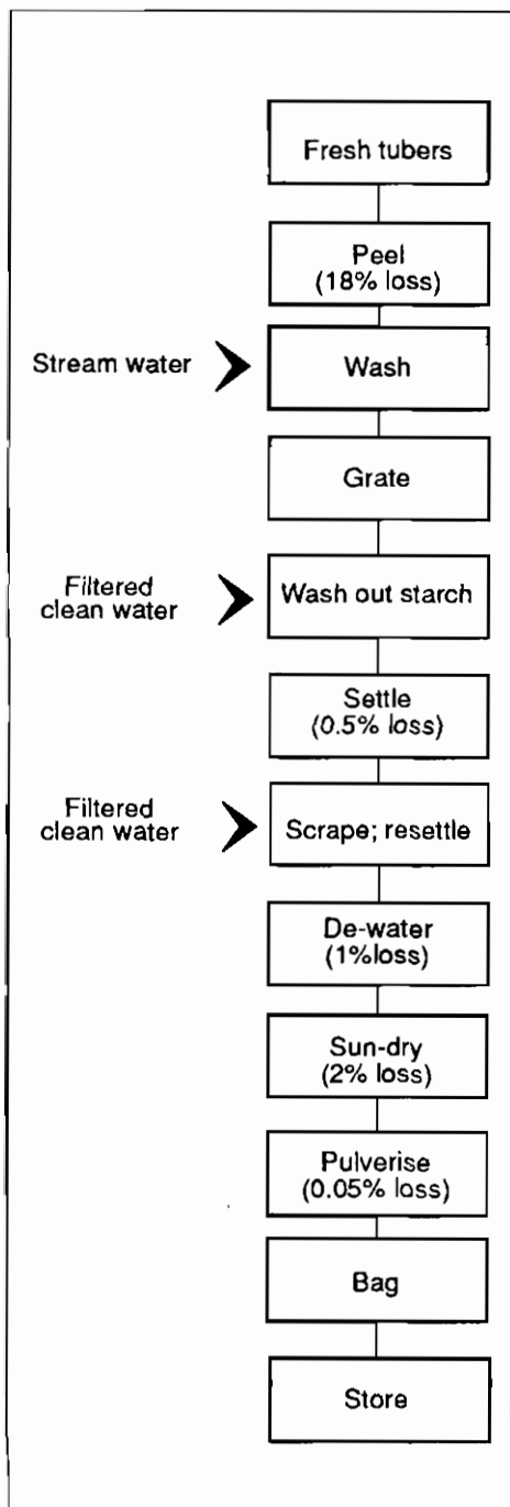
Figure 9.16. Flow chart for manufacture of cassava starch
