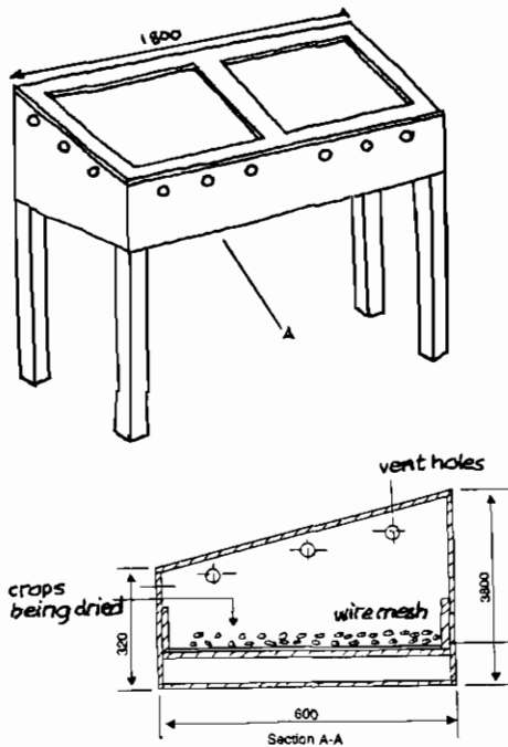
Figure 9.23. Cabinet dryer, showing cross-section (below)
