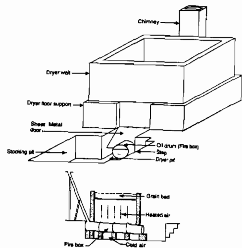
Figure 9.25. Brook dryer, showing cross-section (below)
