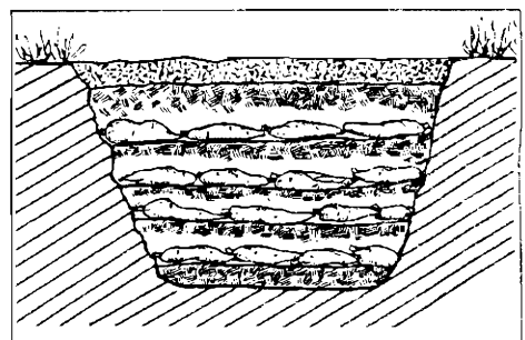
Figure 8.2 Cassava roots stored in a trench, covered with soil
