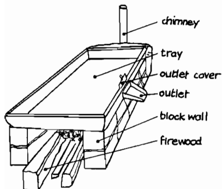
Figure 9.20. RAIDS gari fryer
