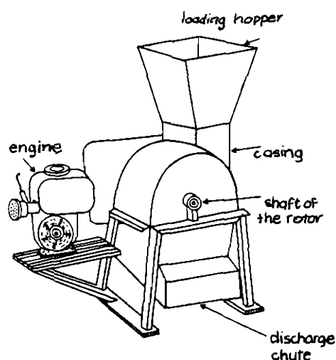
Figure 9.18 A typical cassava grater
