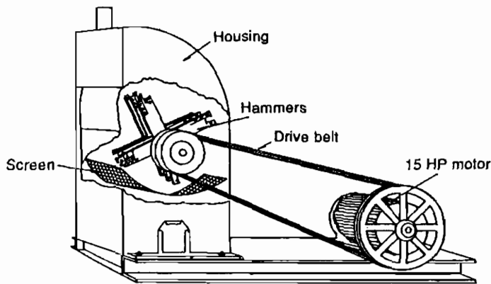
Figure 9.24 Hammer mill
