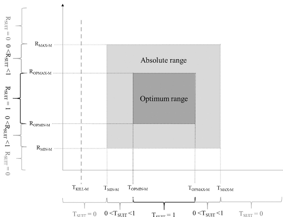
Fig. 2. Ecocrop model, adapted from Ramirez-Villegas et al. (2013). T_{SUIT} = temperature suitability. R_{SUIT} = rainfall suitability. T_{KILL-M} = minimum temperature parameter below which crop dies. T_{MIN-M} = minimum absolute temperature, T_{OPMIN-M} = minimum optimum temperature, T_{OPMAX-M} = maximum optimum temperature, T_{MAX-M} = maximum absolute temperature. R_{MIN-M} = minimum absolute rainfall, R_{OPMIN-M} = minimum optimum rainfall, R_{OPMAX-M} = maximum optimum rainfall, R_{MAX-M} = maximum absolute rainfall.
