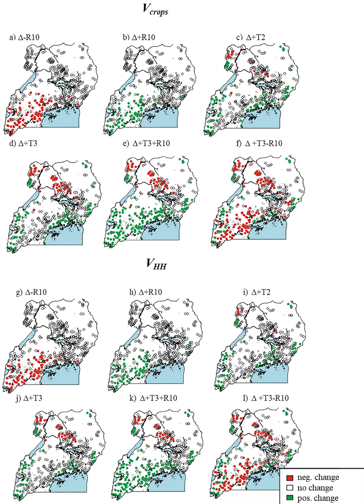
Fig. 6. Household (crop) vulnerability represented by household level crop suitability change ( V_{crops} , a-f) and household level suitability change ( V_{HH} , g-l) under six simplified climate scenarios: Difference between scenario -R10 and current climate (a, g); +R10 and current climate (b, h); +T2 and current climate (c, i); +T3 and current climate (d, j); +T3 + R10 and current climate (e, k); +T3-R10 and current climate (f, l). -10% = 10% monthly rainfall decline, +R10 = 10% monthly rainfall increase, +T3 = 3 °C monthly minimum and mean temperature increase. Negative change: V_{crops} or V_{HH} < -0.05 . Positive change: -V_{crops} or V_{HH} > 0.05 . No change: -0.05 \leq V_{crops} or V_{HH} \leq 0.05 .
