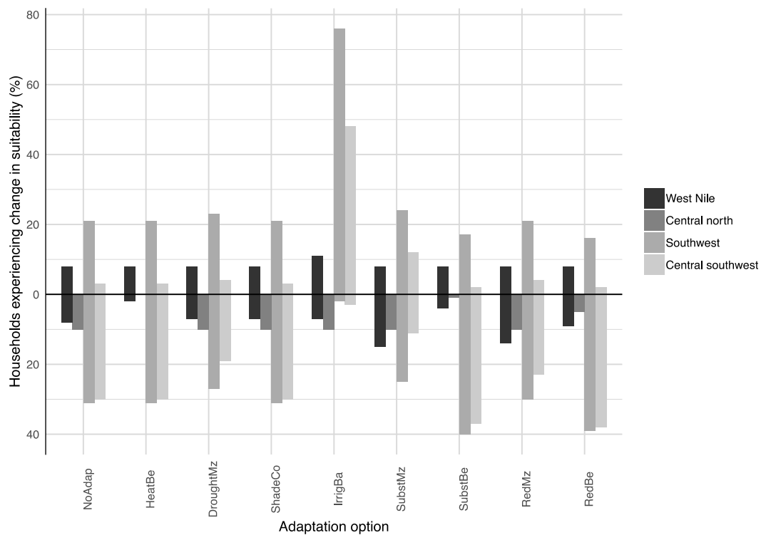
Fig. 8. Percentage of households per hotspot experiencing a negative (bars facing down from the horizontal line) or a positive (upward bars) change in household level suitability due to climate change (3 °C increase and 10% rainfall decrease) compared to current climate and for different adaptation options (For explanation of adaptation options see Table 2).
