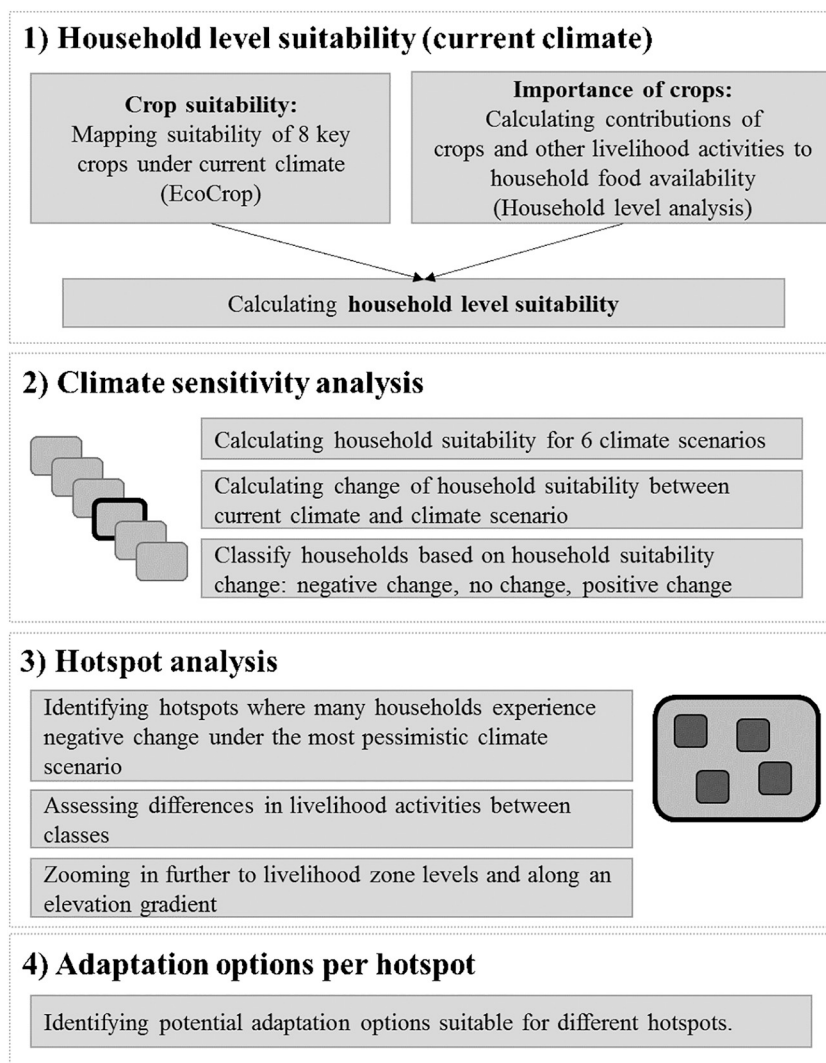
Fig. 1. Schematic overview of the approach, for details see text.
