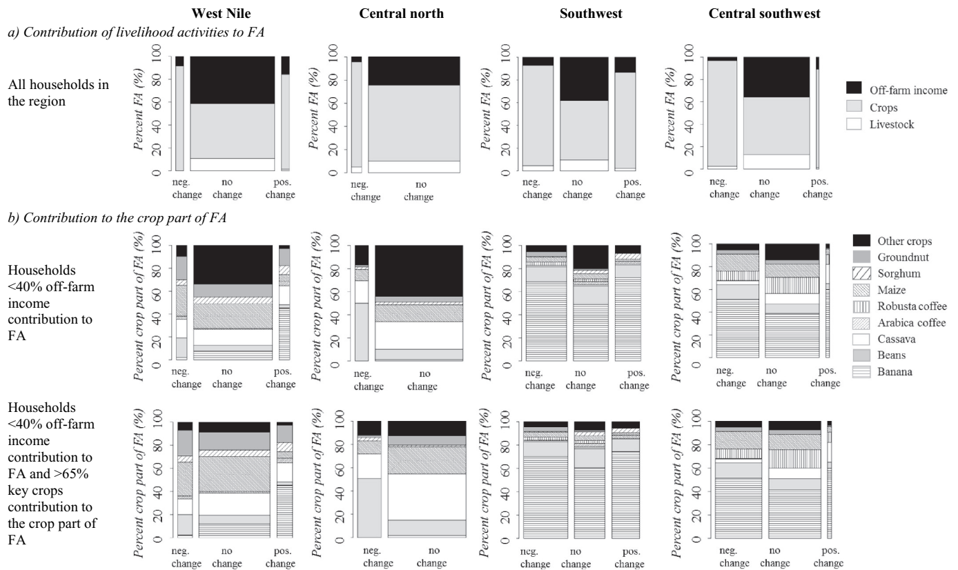
Fig. 7. Livelihood activities (a) and crops (b) contributing to food availability (FA), classified by household level suitability change (neg. change = negative change; no change; pos. Change = positive change) from baseline to scenario +T3-R10 per hotspot (3 °C increase and 10% rainfall decrease compared to baseline). Width of bar represents percentage of households in class. Information on household numbers in SI Table 9.
