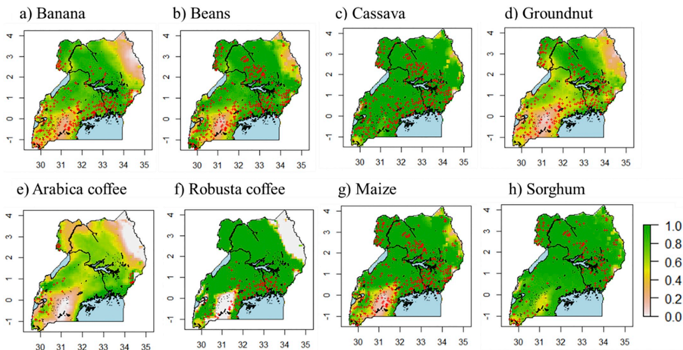
Fig. 3. Crop suitability under current climate for eight key crops based on thresholds of monthly temperature and seasonal rainfall using the Ecocrop model. A suitability score = 1 means highly suitable, a suitability score = 0 means not suitable. The red + represent the households with the particular crop present on their farm. (For interpretation of the references to colour in this figure legend, the reader is referred to the web version of this article.)
