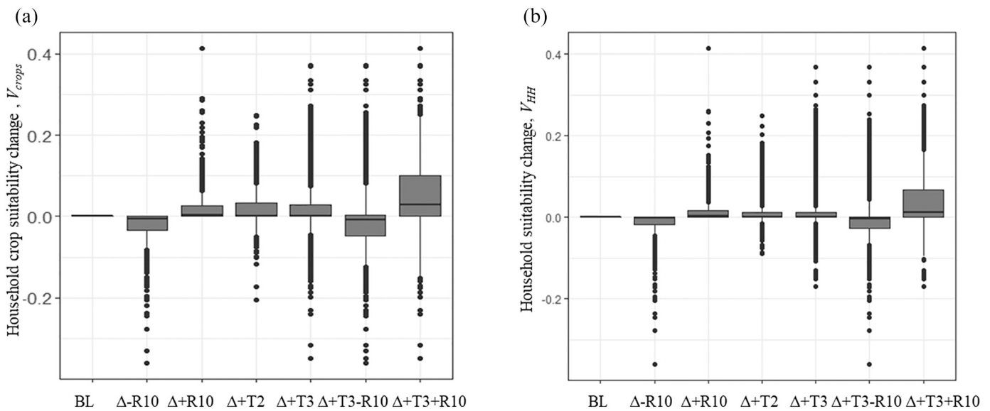
Fig. 5. a) Household crop suitability change ( V_{crops} ) and b) household suitability change ( V_{HH} ) under six simplified climate scenarios for all households across Uganda.
