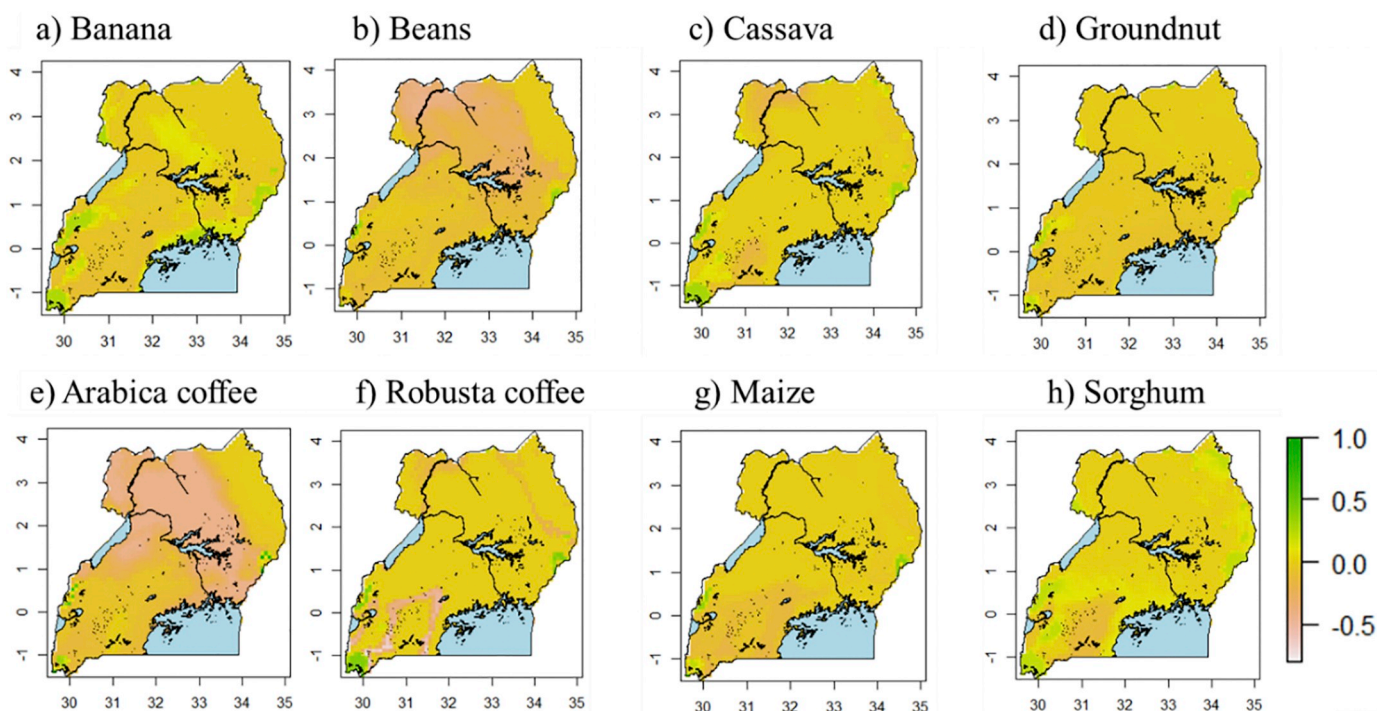
Fig. 4. Change in crop level suitability under climate scenario +T3-R10 compared to current climate (maps show difference = crop level suitability +T3-R10 - crop level suitability base ).
